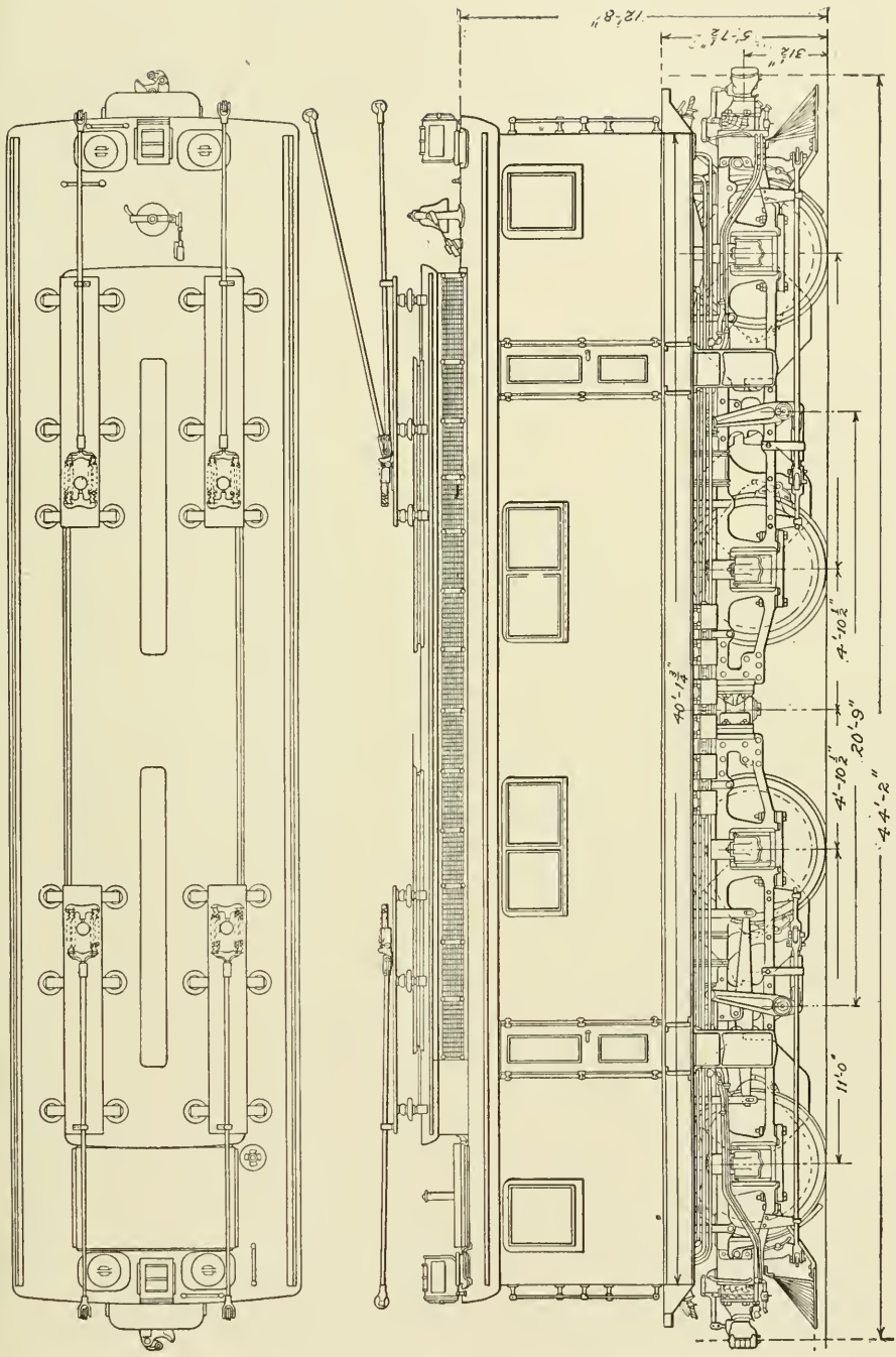
Fig. 267. Plan and Elevation of Great Northern Locomotive
